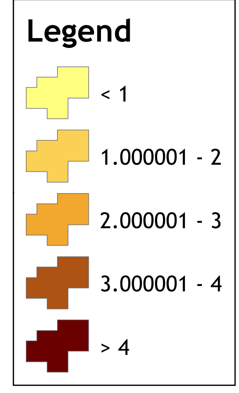
Pick Six
